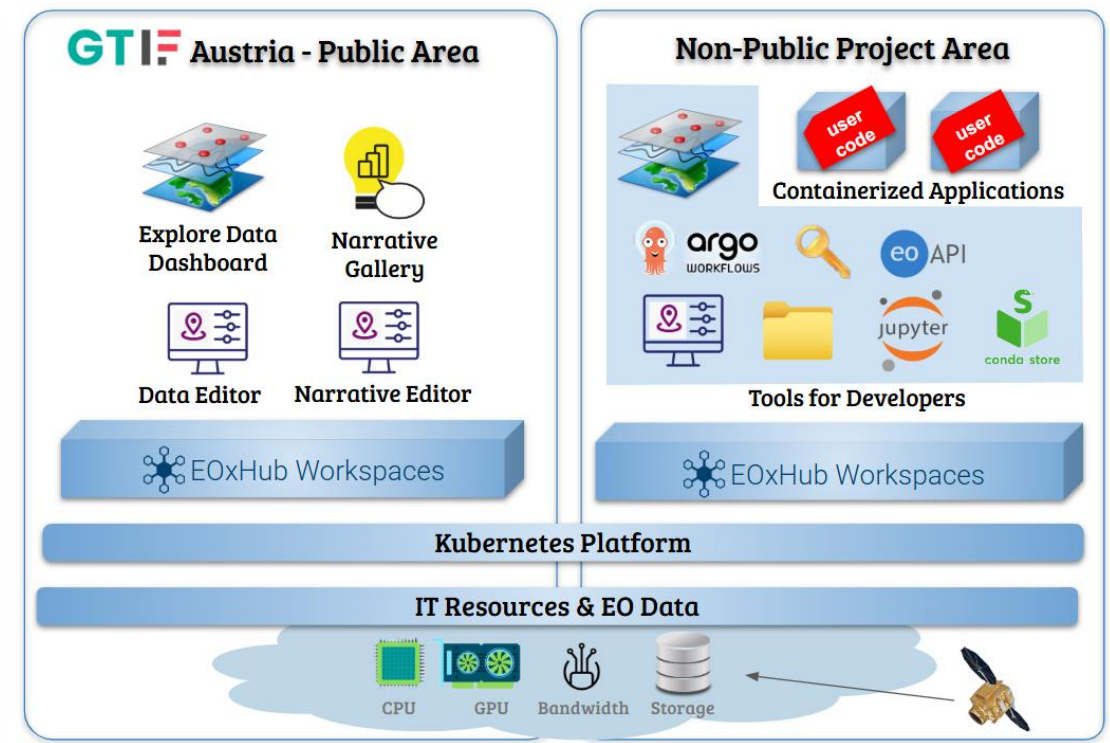
Figure 8 GTIF Architecture
