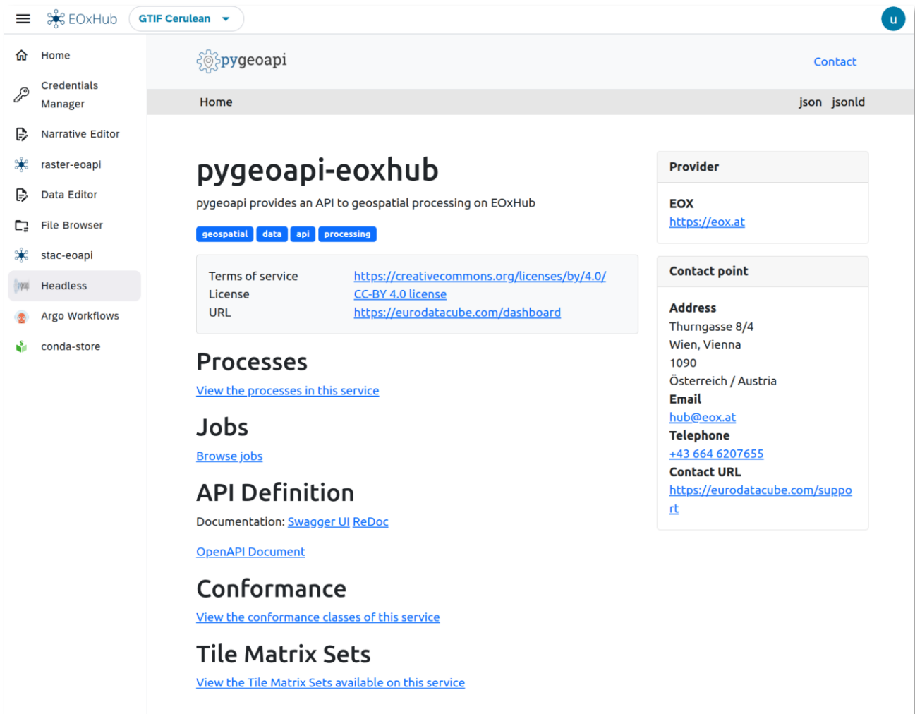
Figure 14 Web interface for the Headless execution feature
